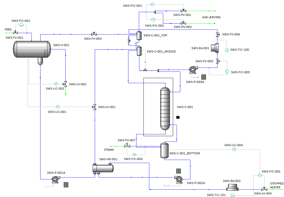
Figure 3. SWS flow sheet for Model B.
