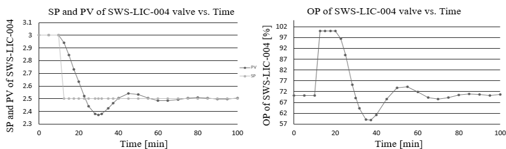
Figure 8. Effect of the level set-point change for the cascade control SWS-LIC-004; a. Changes of the level set-point variable SP and level process variable PV; b. Change of the master controller output (OP).
