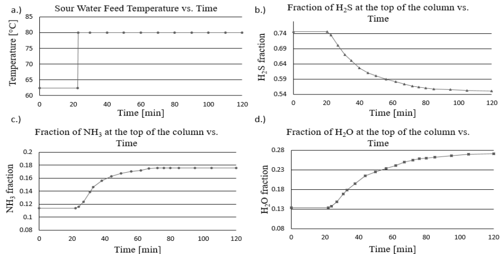
Figure 6. Effects of changing the SWS inlet temperature on the mass fraction of the components at the top of the column.
