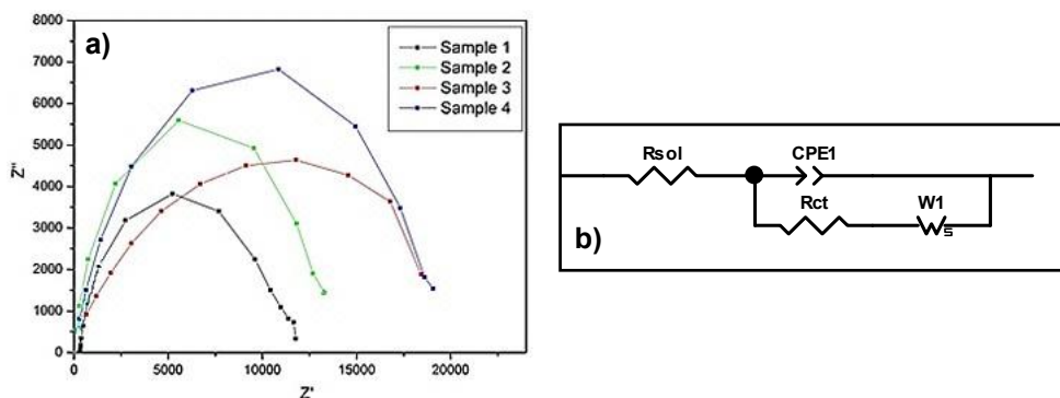
Fig. 6. Nyquist plot (a) and equivalent circuit for spectra modeling (b)
